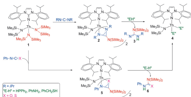
Scheme 1. Reactions of [\text{Th}(\text{Im}^{\text{Dipp}}\text{N})\{\text{N}(\text{SiMe}_3)_2\}_3] ( 1 ) with stoichiometric amounts of heterocumulenes.
