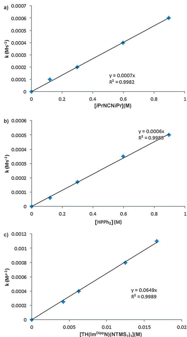
Figure 1. Plot of reaction rate \partial p/\partial t against the concentration of a) DIC for the reaction of DIC and HPPPh 2 ; b) HPPPh 2 for the reaction of DIC and HPPPh 2 ; c) of complex 1 .
